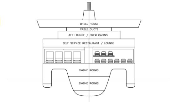
CROSS SECTION
